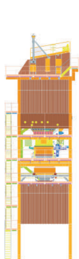
S tower and G tower with same configuration and drawn in the same scale
