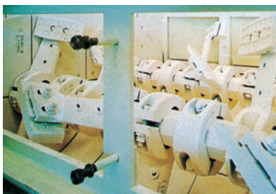
Twin shaft paddle mixer. Designed for low power consumption and low wear. Heated by thermal oil. High resistance wearing parts. Equipped with lateral access gates for an easy replacement of paddles, etc.
